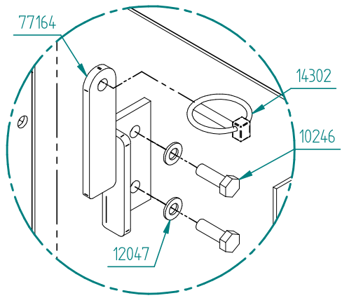
DETAIL C
